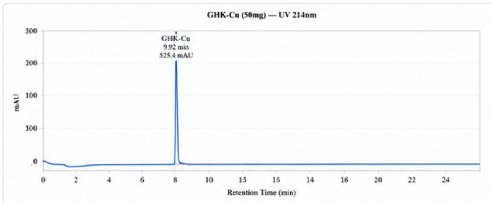
HPLC Chromatogram
