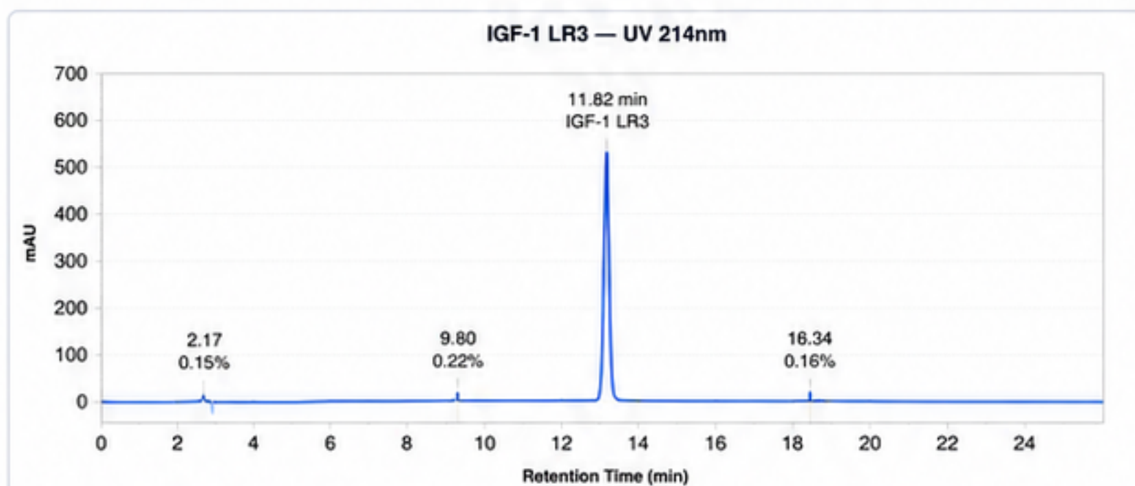
HPLC Chromatogram
