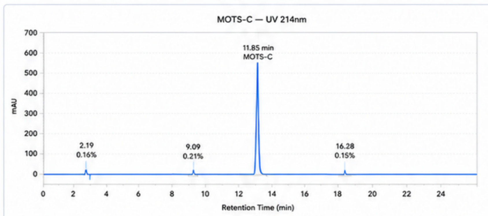
HPLC Chromatogram
