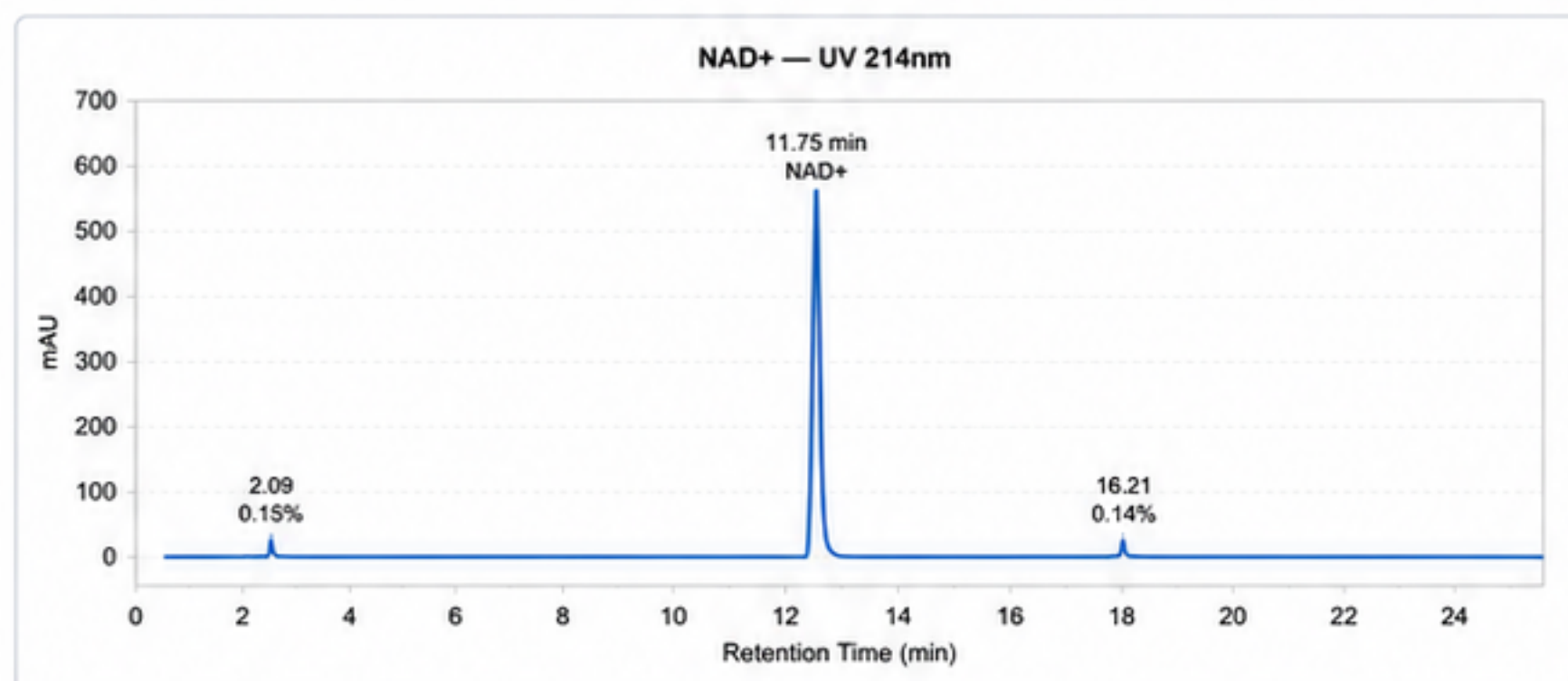
HPLC Chromatogram
