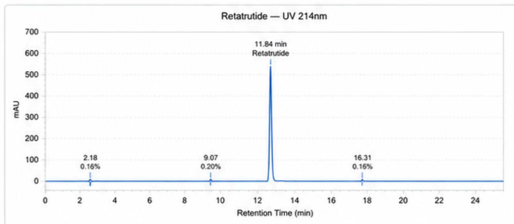
HPLC Chromatogram
