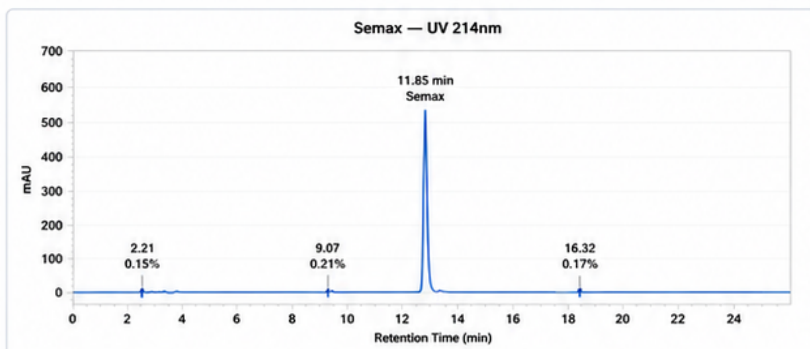
HPLC Chromatogram
