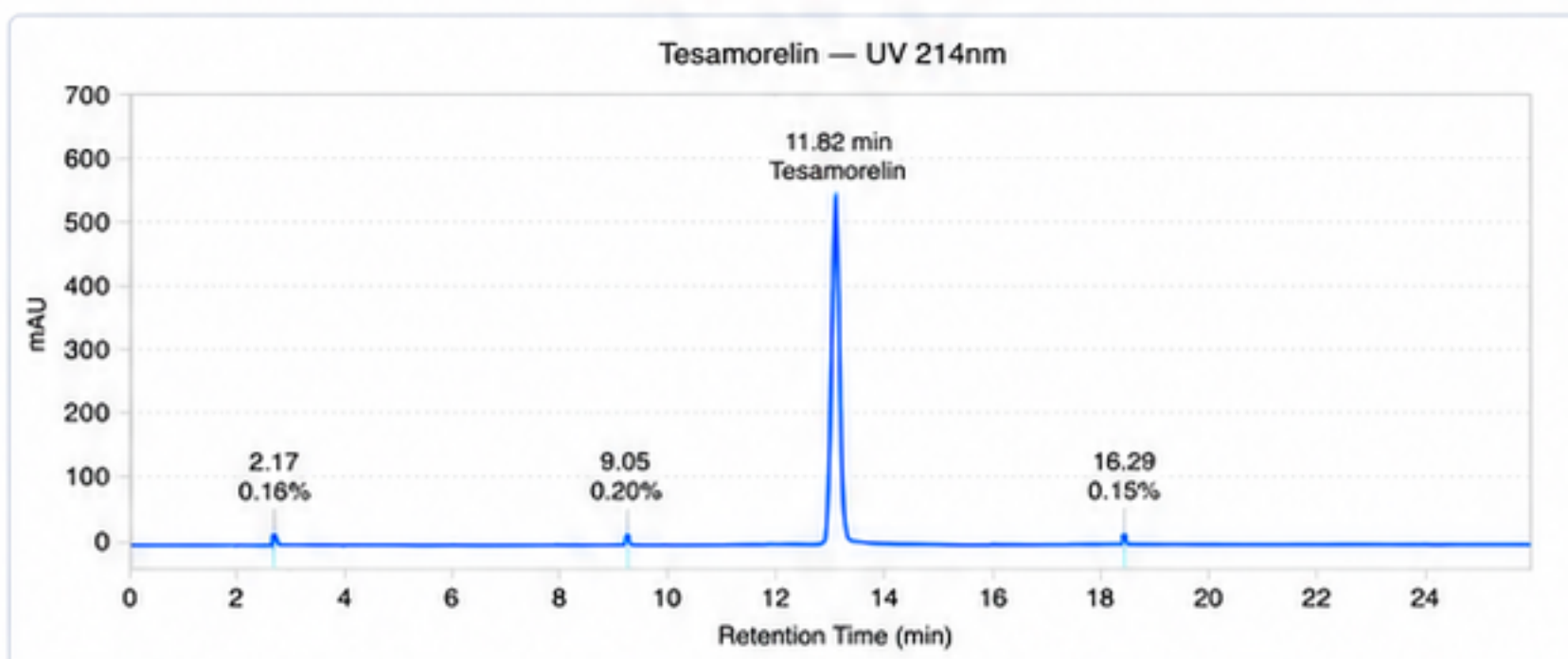
HPLC Chromatogram
