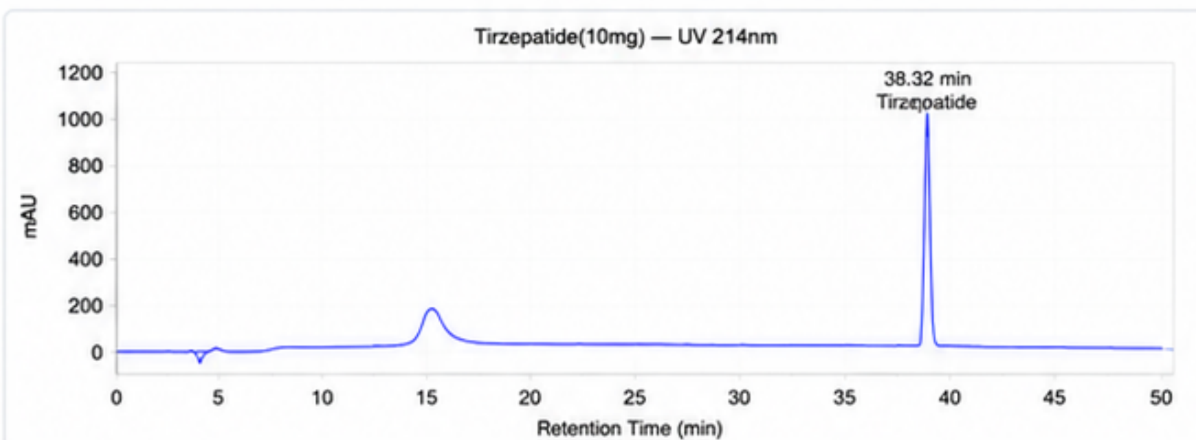
HPLC Chromatogram
